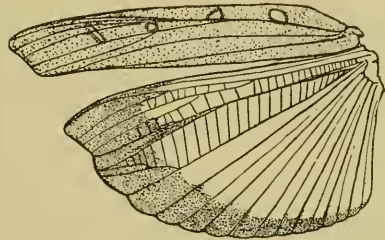
FIG. 5.— AOLACRIS BELLA . TEGMEN AND WING (X 1)
